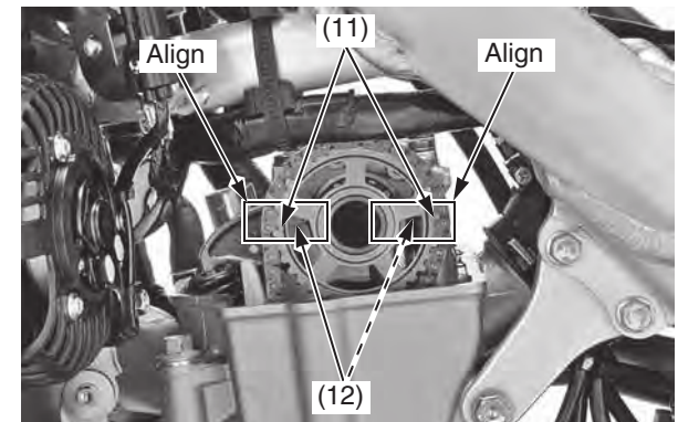
(11) timing mark (12) camshaft holder mating surface
