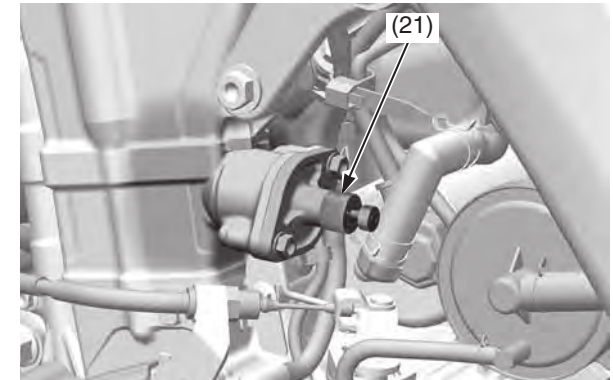
(21) tensioner stopper
