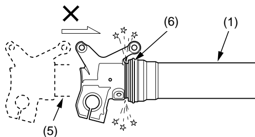
(1) outer tube (5) slider (6) dust seal
