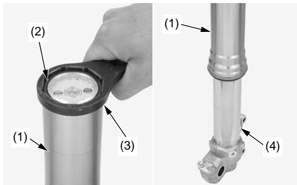
(1) outer tube (2) fork damper (3) lock nut wrench (4) axle holder
