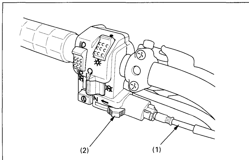
(2) Choke lever
