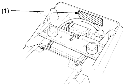
(1) vehicle emission control information label
