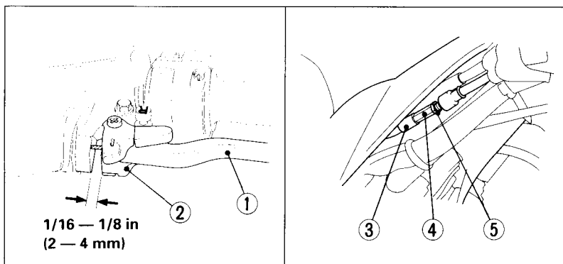
Fig. 4-18 (1) Rear brake lever (2) Reverse assist lever (3) Rubber sleeve (4) Adjusting nut (5) Lock nut
