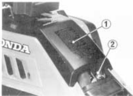
(1) Air cleaner case top cover (2) Wing bolt
