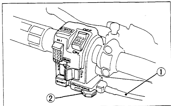
(2) Choke lever
