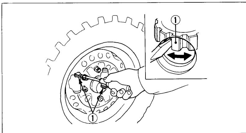
(1) Brake adjusters
