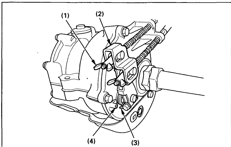
Fig. 4-27 (1) Brake lever adjusting nut (2) Brake arm (3) Arrow (4) Reference mark
