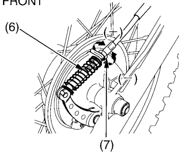
(6) lower lock nut
